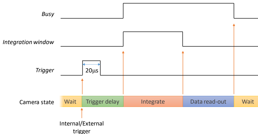
Figure 10 Busy , Integration window and Trigger output functions.
