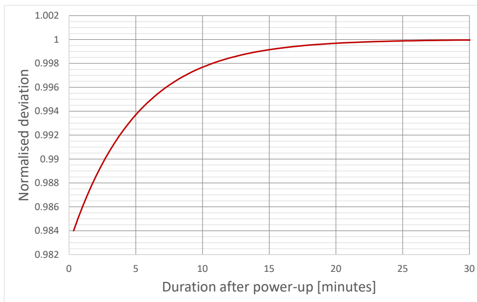
Figure 14 Drift after power-up.
